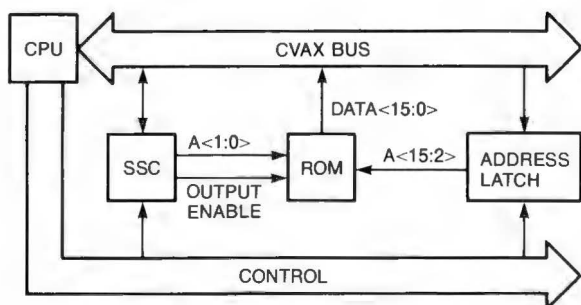
Figure 2 SSC ROM Packing Connection Diagram
