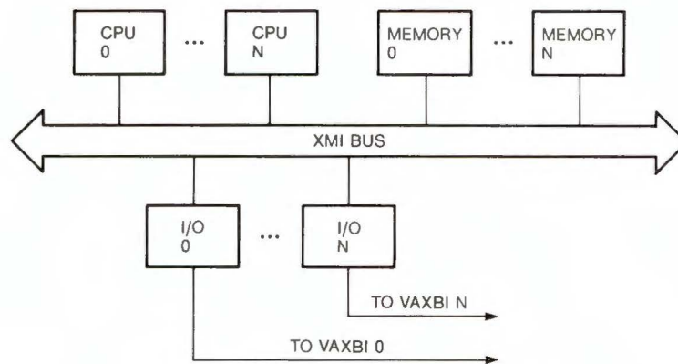
Figure 1 VAX 6200 System Architecture
