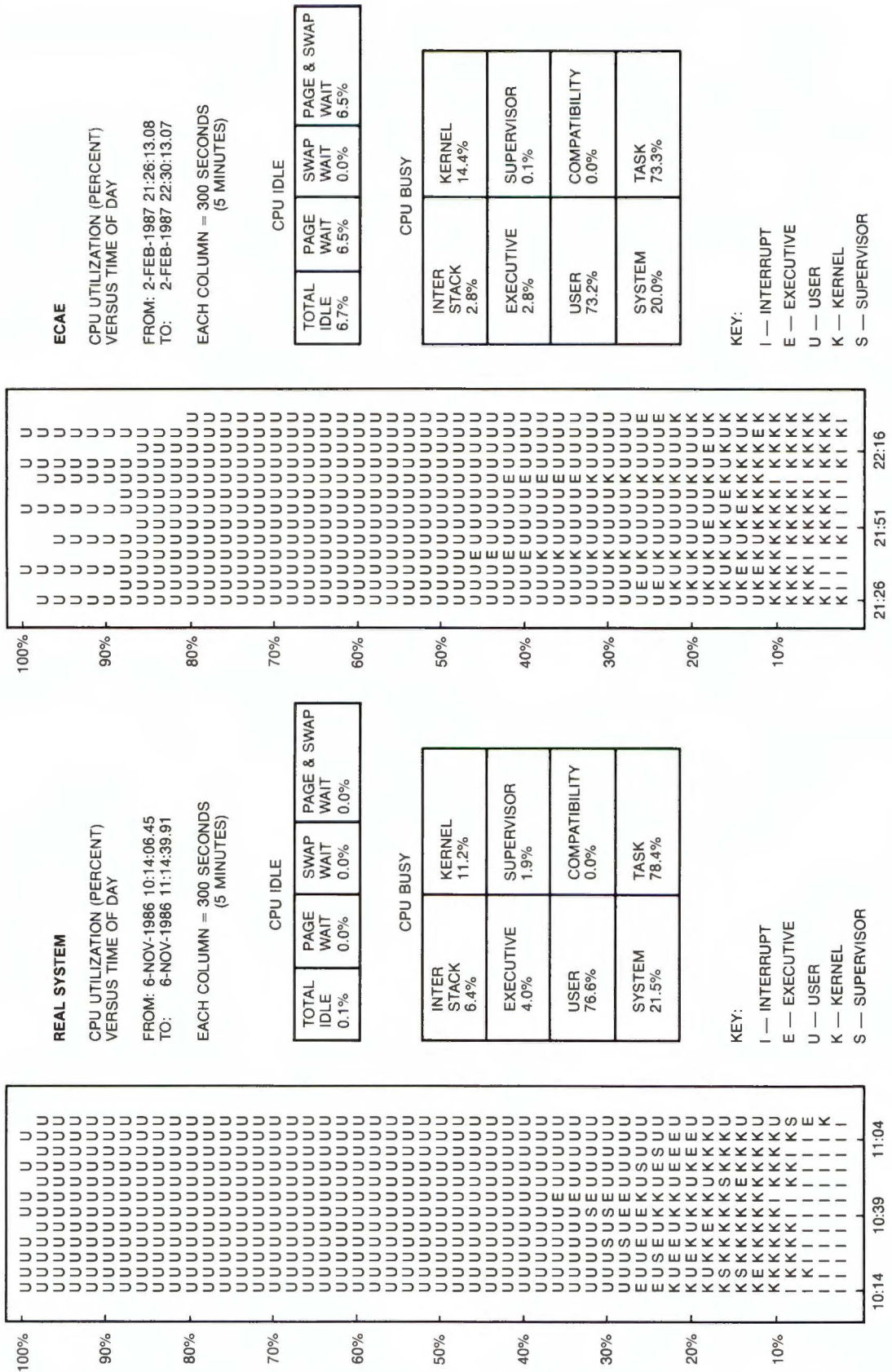
Figure 3 CPU Utilization for Real Internal System and ECAE Workload for 1 Hour
