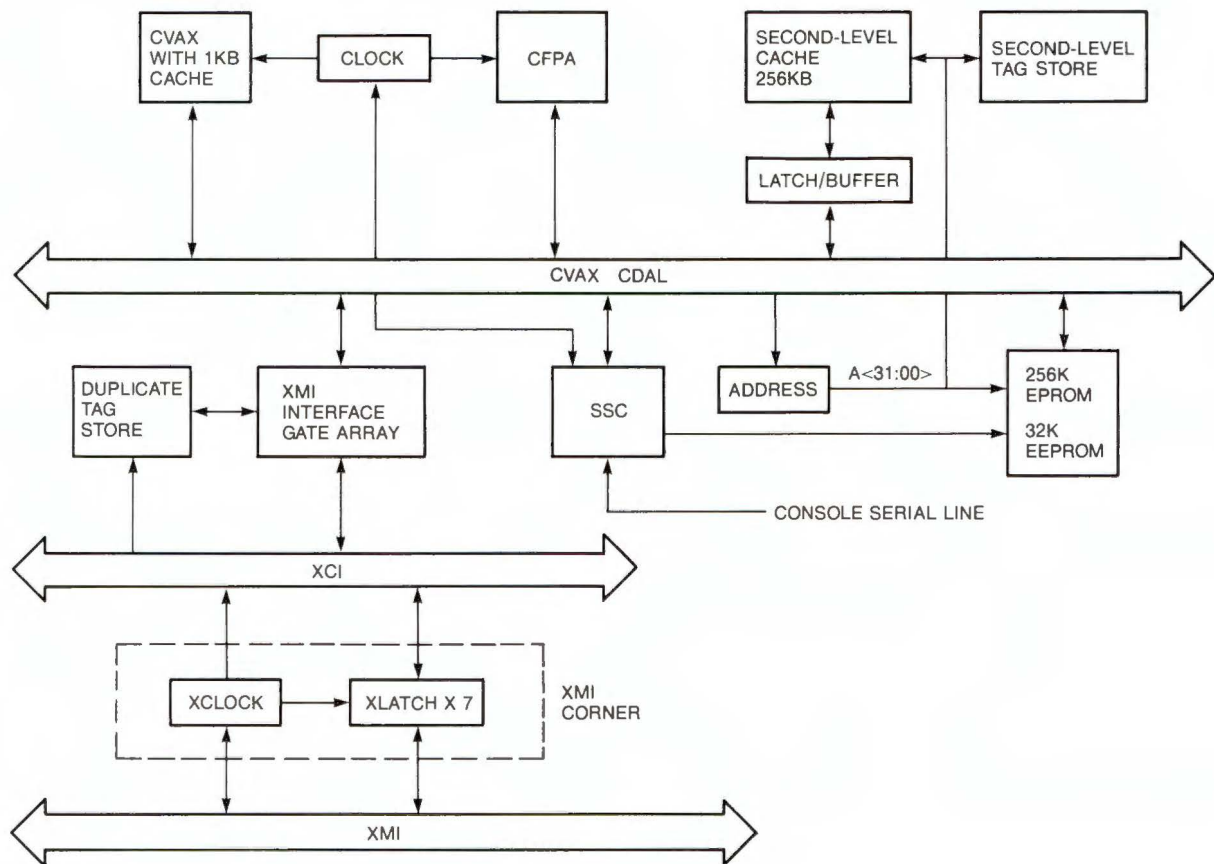
Figure 4 VAX 6200 CPU Block Diagram
