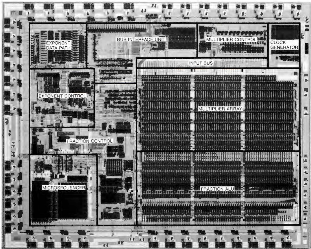
Figure 3 CFPA Physical Layout
