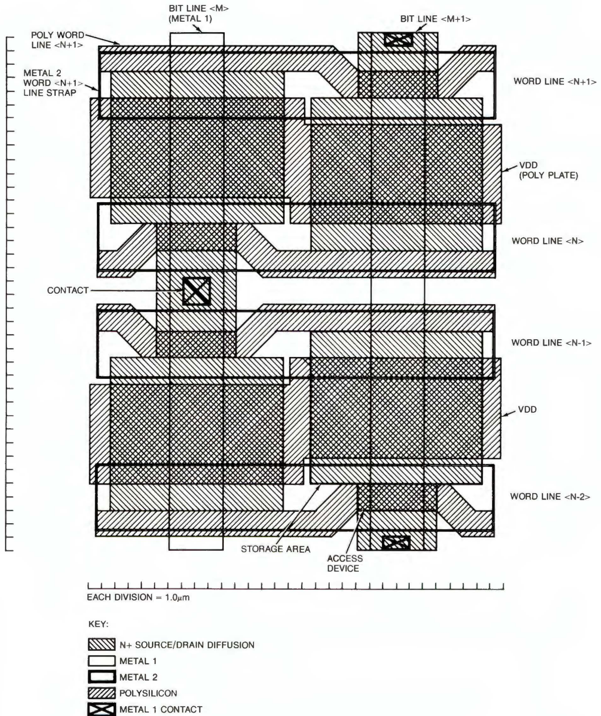
Figure 4 Cache 1T Dynamic RAM Cell (Four Cell Shown)
